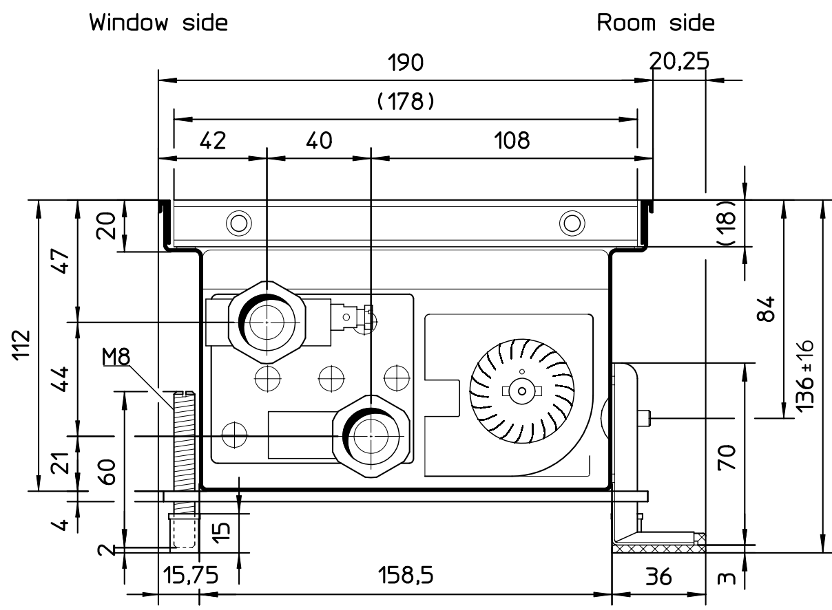
Cross-sections (enlarged) showing roll-up grille
