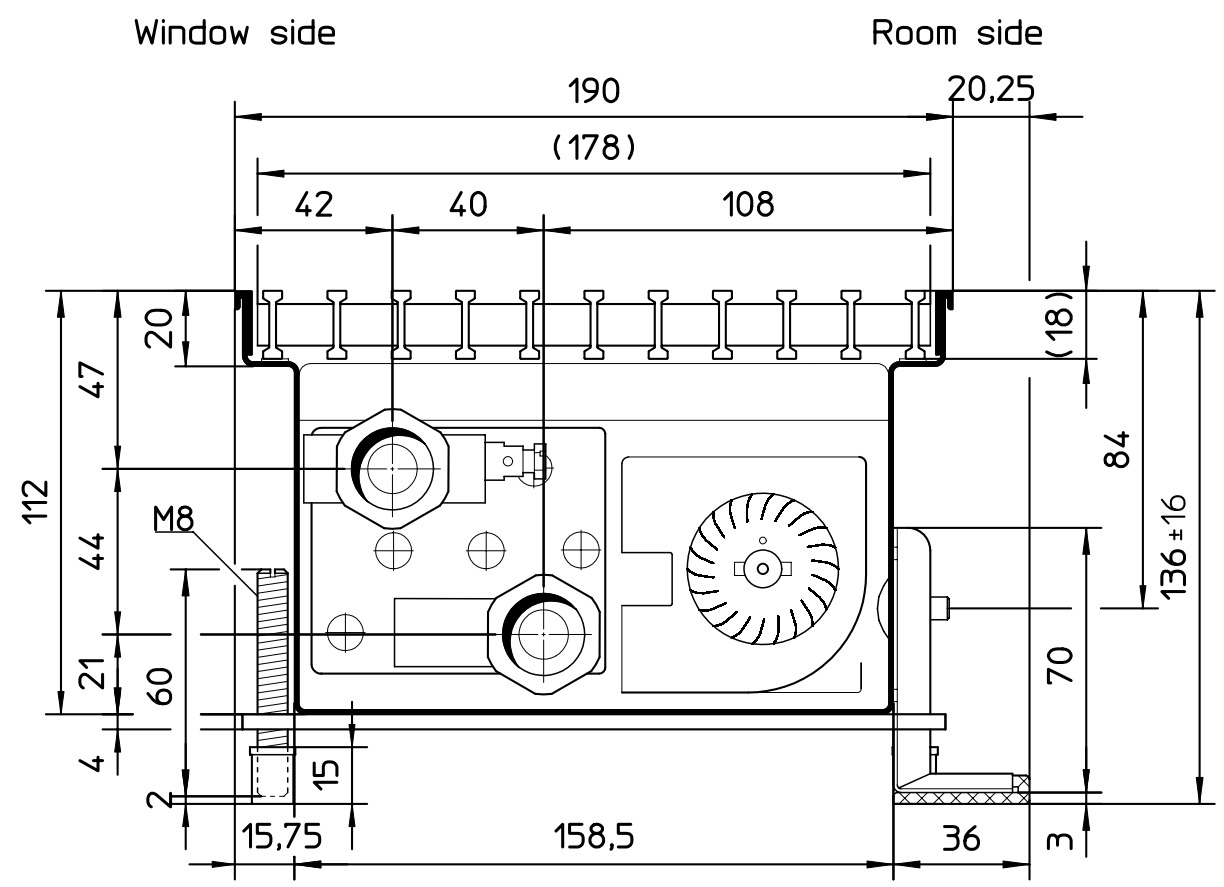
Cross-sections (enlarged) showing linear grille
